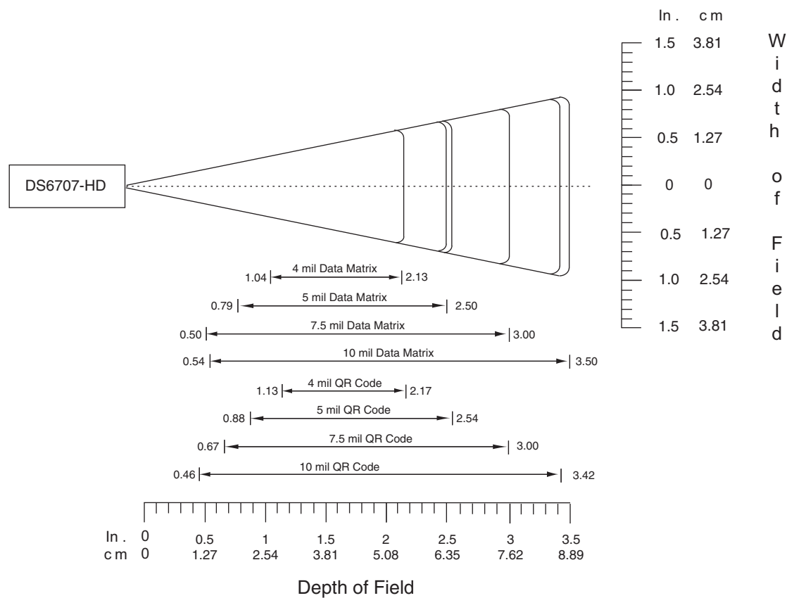
Figure 2-15 DS6707-HD High Density Digital Imager Scanner Decode Zone for 2D Bar Codes
